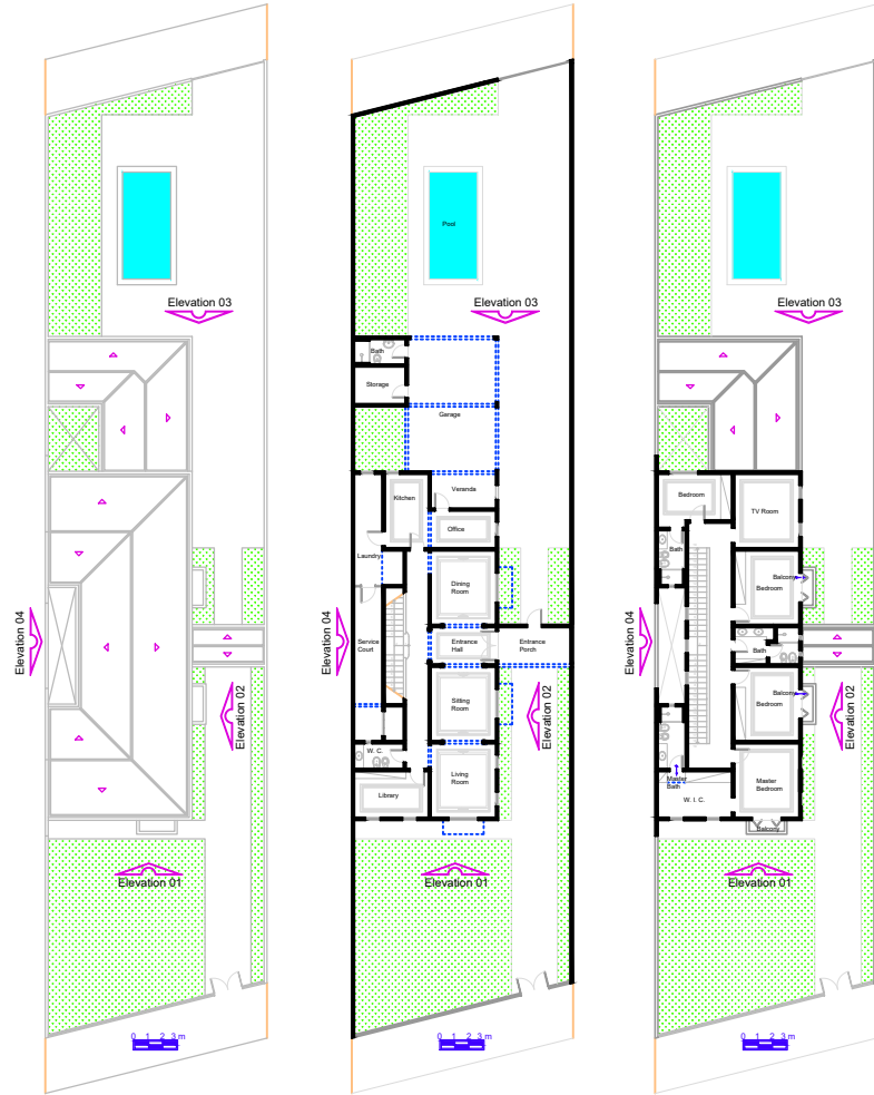
First Floor Plan A = 197,06 m 2
